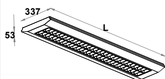
drawing OPAL + LOUVER
